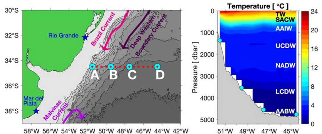
Figure 1. (left) Map indicating the locations of the four PIES moorings (large cyan circles) and the nominal locations of the CTD profiles collected on routine research cruises (red dots). PIES site names are denoted by large white letters. Bottom topography from the Smith and Sandwell (1997) data set is shown as gray-filled contours with a 500 m contour interval. Simple schematic arrows indicating the locations of the nearby major ocean currents are included to illustrate the array position relative to the large-scale flow features; schematic modified from Valla et al. (2018). (right) Vertical section of temperature (averaged from four CTD sections during 2009–2012) along the PIES mooring line. PIES locations are shown as cyan circles. Nominal central depths of key water mass layers denoted by acronyms following Valla et al. (2018). TW = Tropical Water; SACW = South Atlantic Central Water; AAIW = Antarctic Intermediate Water; UCDW = Upper Circumpolar Deep Water; NADW = North Atlantic Deep Water; LCDW = Lower Circumpolar Deep Water; AABW = Antarctic Bottom Water.
