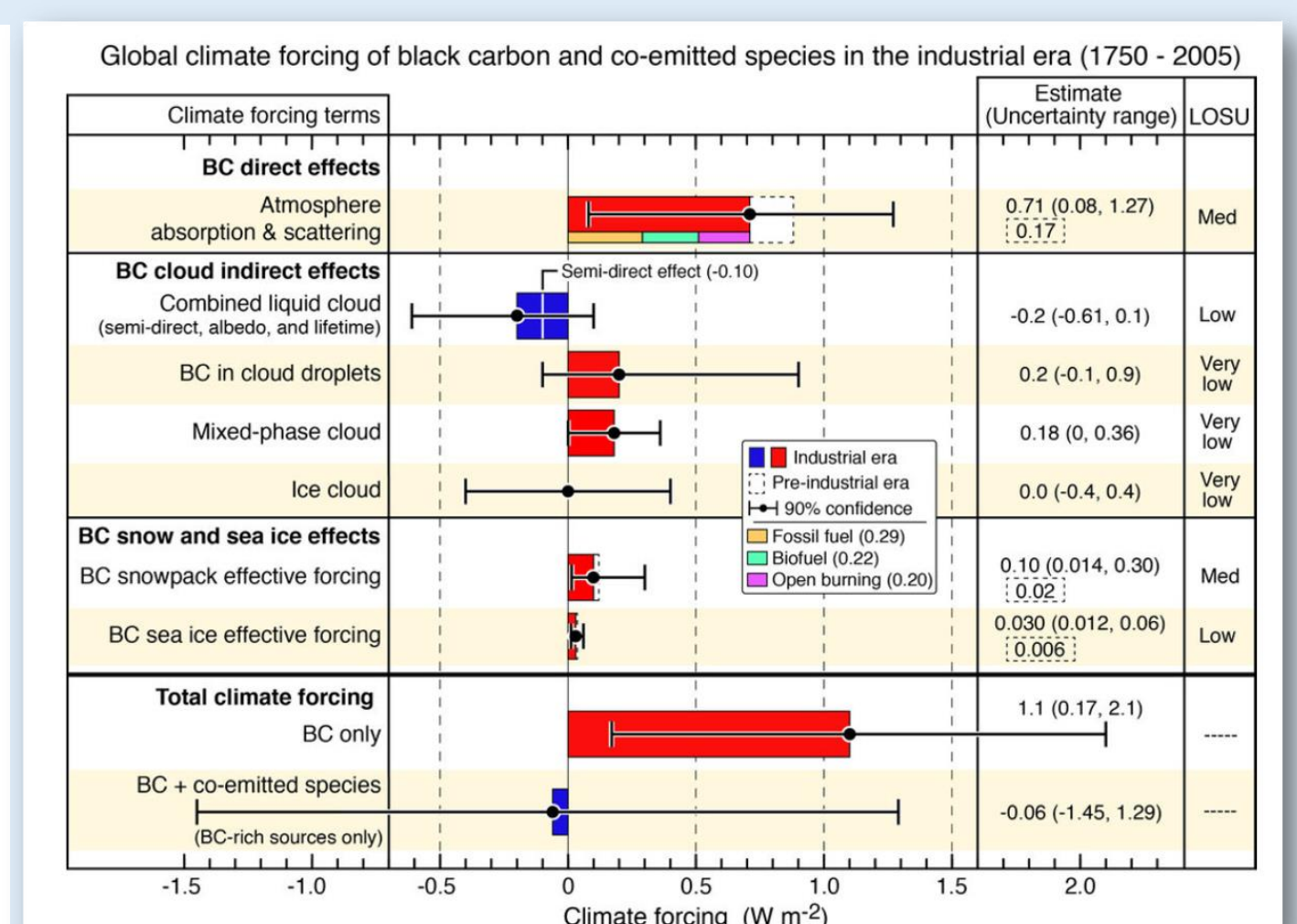
Fig.4- Bond et al. 2013, estimates the same forcing of the BC in +1.1 w / m 2 , extremely high value, and if we take into account co-emitted particles, the forcing is -0.06 w / m 2 .
