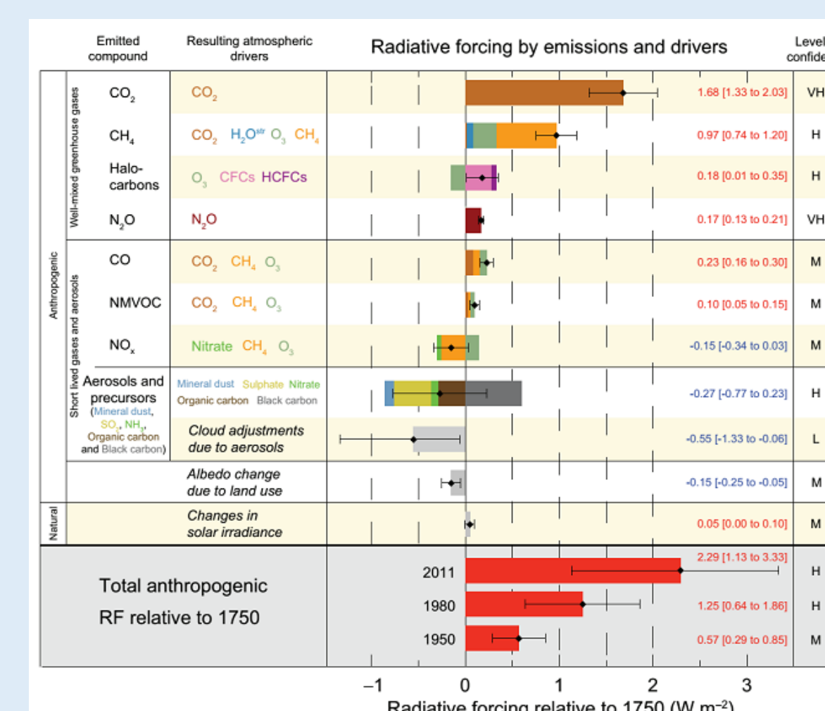
Fig.3 - The BC is important for the global radiative forcing (IPCC 2013), and according to the last report it accounts for about +0.65 w / m 2 .
