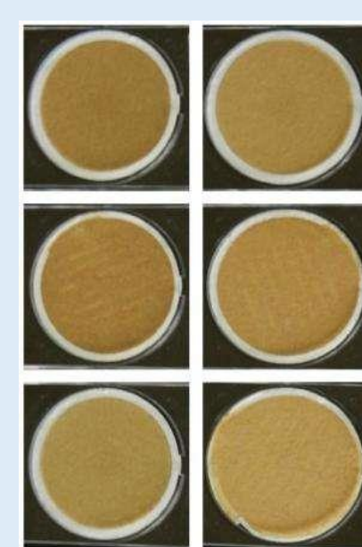
Fig.2- Samples of BrC obtained during the 6 hour period next to a burning funeral pyre in India. Chakrabarty, 2014.
