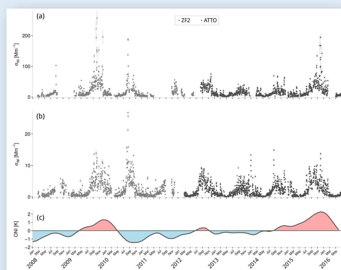
Fig.7 - In situ aerosol light scattering and absorption at the ZF2 and ATTO sites in Central Amazonia. The time series spans from 2008 to 2016. The third variable is the El-Nino index showing the oscillation between El Nino and La Nina over the same period. The single scattering albedo also changes significantly. No Brown Carbon measurements is being done so far in Amazonia.
